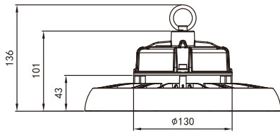
01 YL-HB01-100W
