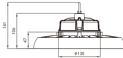
02 YL-HB01-150W
