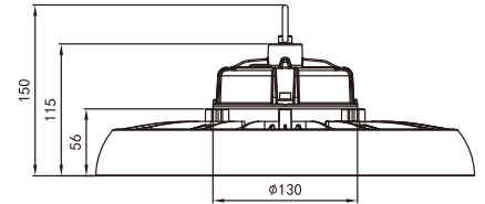
03 YL-HB01-200W /YL-HB01-240W
